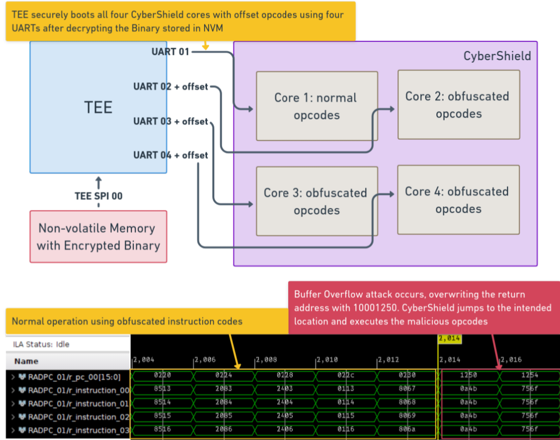
Figure 7: Diagram of RadPC + TEE (CyberShield) with ILA outputs. The block diagram shows the TEE bootloading each RadPcC core with their respective offsets. Core 1 runs normal RISC-V opcodes, while Cores 2-4 run opcodes with unique offsets. This can be seen in the ILA. When the buffer overflow attack occurs all four cores have the same opcodes which is an IoC.
