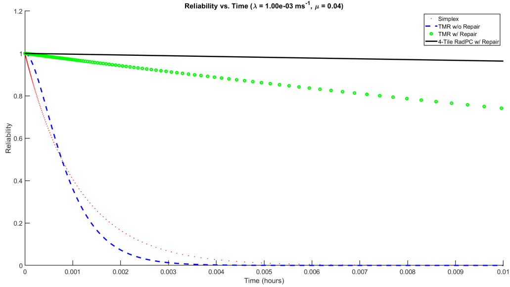
Fig. 7 Exponential reliability curve for 4-Tile RadPC system with repair capability
