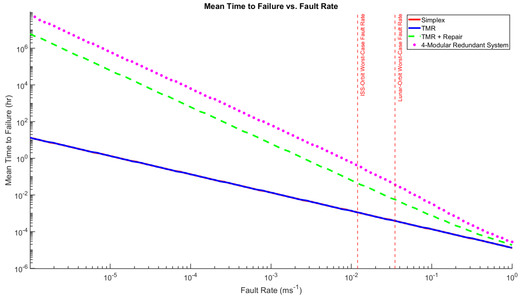
Fig. 10 MMTF versus fault rate for varying architectures
