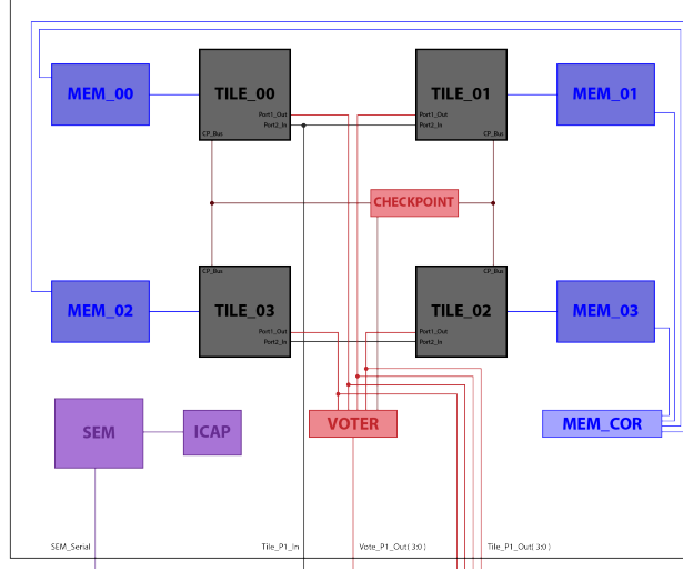
Fig. 2 Block Diagram of RadPC Architecture
