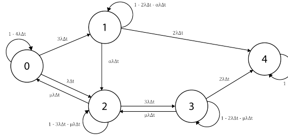
Fig. 6 Markov chain model state diagram for a TMR + PR + SEM + Spare Tile System
