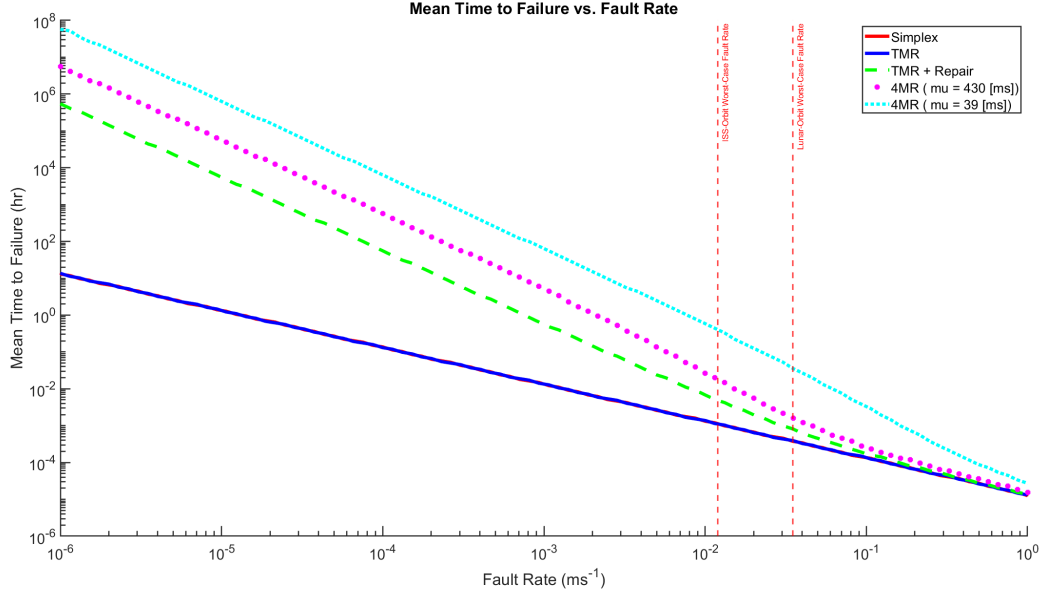
Fig. 12 MMTF versus fault rate for varying architectures, best-performing \mu for 4MR system
