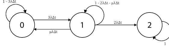
Fig. 4 Markov chain model state diagram for a TMR system
