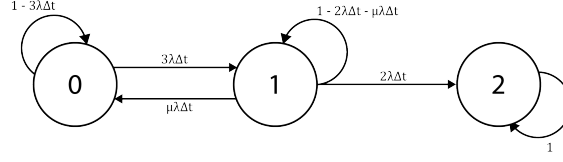
Fig. 5 Markov chain model state diagram for a TMR + PR + SEM system
